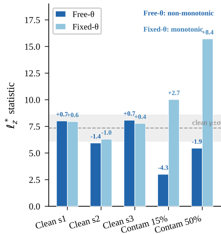
(a) \ell_z^* under Free- \theta vs Fixed- \theta
