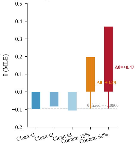
(c) \theta -Shift Mechanism
