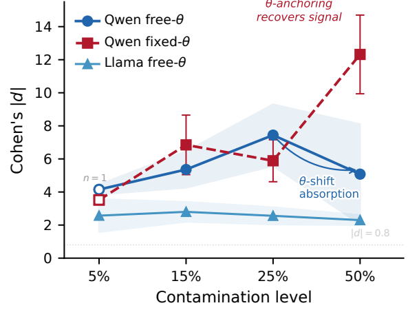
Figure 3: Dose-response trajectories on MMLU. Free- \theta (solid) shows non-monotonic behavior for Qwen due to \theta -shift absorption (shaded); fixed- \theta (dashed) removes the inverted-U artifact and yields an overall positive dose-response ( |d|=12.32 at 50%). Llama’s flat trajectory reflects minimal absorption. Hollow markers: single-seed ( n=1 ); error bars: \pm SD ( n=3 ).
