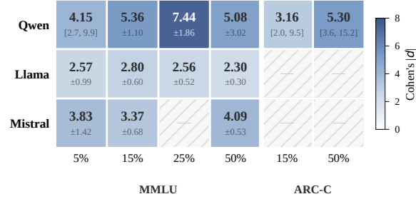
Figure 4: Cohen’s |d| heatmap (values from Table 1; multi-seed means where available). Blue intensity reflects effect-size magnitude. Grey cells: not tested.
