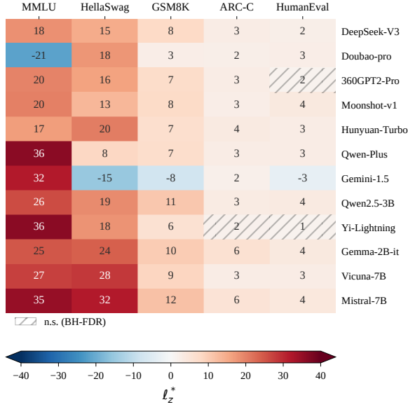
Figure 5: \ell_z^* heatmap for 12 leaderboard models across five benchmarks. 57/60 cells exceed |\ell_z^*| > 1.96 , indicating pervasive IRT assumption violations even absent contamination. Details in Appendix E.
