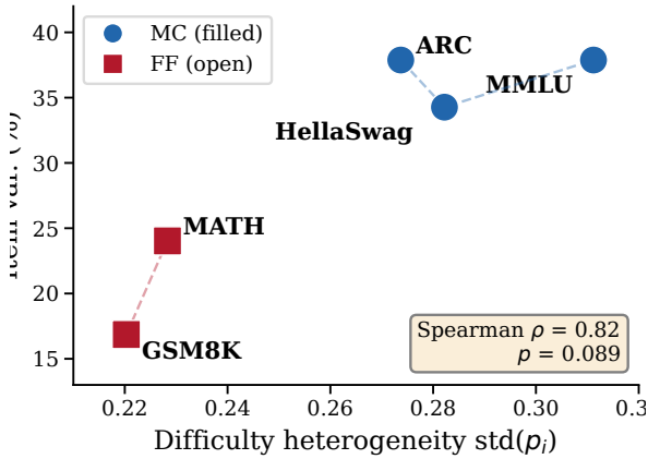
Figure 8: Item difficulty heterogeneity ( \text{std}(p_i) ) versus \text{item\_id} variance share across five benchmarks. MC benchmarks (filled) exhibit higher difficulty dispersion and item variance than FF benchmarks (open). Spearman \rho = 0.82 .
