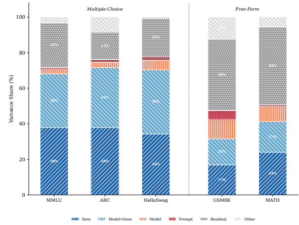
Figure 9: Variance decomposition (Henderson Method I) across five benchmarks and eight models. Multiple-choice benchmarks share an item-dominated structure; HellaSwag is the exception where \text{model} \times \text{item} (36.0%) exceeds item difficulty (34.3%). Free-form benchmarks (GSM8K, MATH) distribute variance across item, model, and interaction components with no single dominant source.
