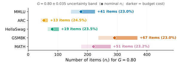
Figure 10: Effect of |\Delta G| = 0.035 estimation error on item budgets. The ~23% increase is consistent across benchmarks.
