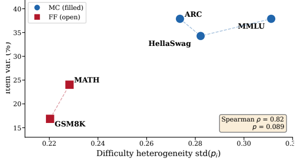
Figure 7: Item difficulty heterogeneity ( \text{std}(p_i) ) versus \text{item\_id} variance share across five benchmarks. MC benchmarks (filled) exhibit higher difficulty dispersion and item variance than FF benchmarks (open). Spearman \rho = 0.82 .
