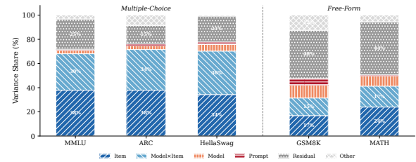
Figure 3: Variance decomposition (Henderson Method I) across five benchmarks and eight models. Multiple-choice benchmarks share an item-dominated structure; HellaSwag is the exception where model×item (36.0%) exceeds item difficulty (34.3%). Free-form benchmarks (GSM8K, MATH) distribute variance across item, model, and interaction components with no single dominant source.
