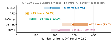
Figure 4: Effect of |\Delta G| = 0.035 estimation error on item budgets across five benchmarks. The \sim 23\% budget increase is consistent across all benchmarks, indicating D-study budgets are robust to estimation uncertainty.
