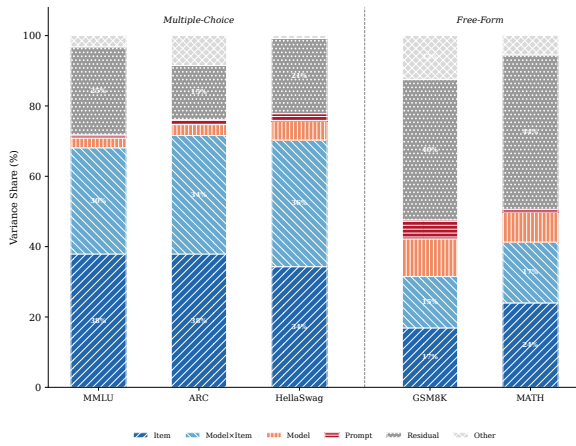
Figure 8: Variance decomposition (Henderson Method I) across five benchmarks and eight models. Multiple-choice benchmarks share an item-dominated structure; HellaSwag is the exception where model \times item (36.0%) exceeds item difficulty (34.3%). Free-form benchmarks (GSM8K, MATH) distribute variance across item, model, and interaction components with no single dominant source.
