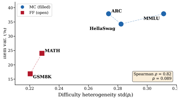
Figure 7: Item difficulty heterogeneity ( \text{std}(p_i) ) versus item_id variance share across five benchmarks. MC benchmarks (filled) exhibit higher difficulty dispersion and item variance than FF benchmarks (open). Spearman \rho = 0.82 .
