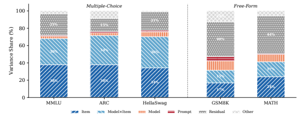
Figure 9: Variance decomposition (Henderson Method I) across five benchmarks and eight models. Multiple-choice benchmarks share an item-dominated structure; HellaSwag is the exception where \text{model} \times \text{item} (36.0%) exceeds item difficulty (34.3%). Free-form benchmarks (GSM8K, MATH) distribute variance across item, model, and interaction components with no single dominant source.
