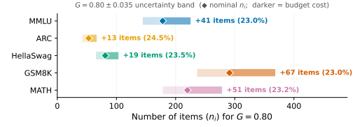
Figure 10: Effect of |\Delta G| = 0.035 estimation error on item budgets. The ~23% increase is consistent across benchmarks.
