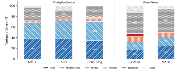
Figure 5: Variance decomposition (Henderson Method I) across five benchmarks and eight models. Multiple-choice benchmarks share an item-dominated structure; HellaSwag is the exception where model \times item (36.0%) exceeds item difficulty (34.3%). Free-form benchmarks (GSM8K, MATH) distribute variance across item, model, and interaction components with no single dominant source.
