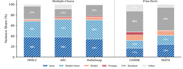
Figure 4: Variance decomposition (Henderson Method I) across five benchmarks and eight models. Multiple-choice benchmarks share an item-dominated structure; HellaSwag is the exception where model \times item (36.0%) exceeds item difficulty (34.3%). Free-form benchmarks (GSM8K, MATH) distribute variance across item, model, and interaction components with no single dominant source.
