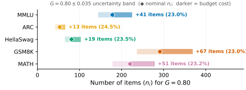
Figure 5: Effect of |\Delta G| = 0.035 estimation error on item budgets across five benchmarks. The \sim 23\% budget increase is consistent across all benchmarks, indicating D-study budgets are robust to estimation uncertainty.
