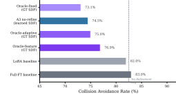
Figure 3: CAR for oracle SDF refinement versus unrefined baselines. All GT oracle variants underperform baselines despite perfect distance information.
