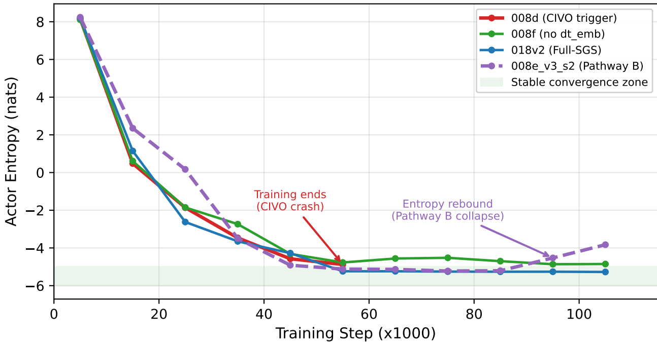
Figure 3: Actor Entropy Dynamics Across Collapse Pathways
