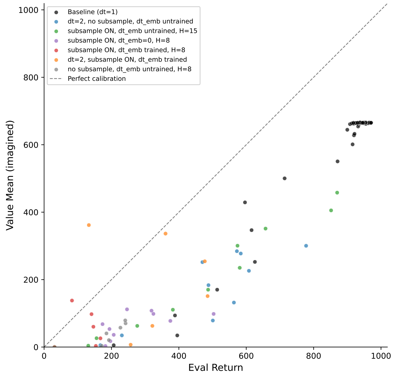
Value Calibration: Value Mean vs Eval Return
