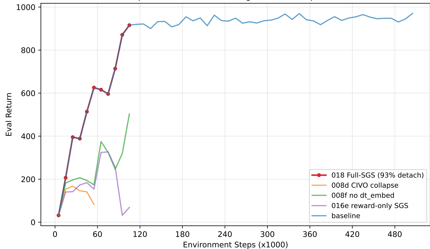
Exp-018 Full-SGS: Learning Curves Comparison
