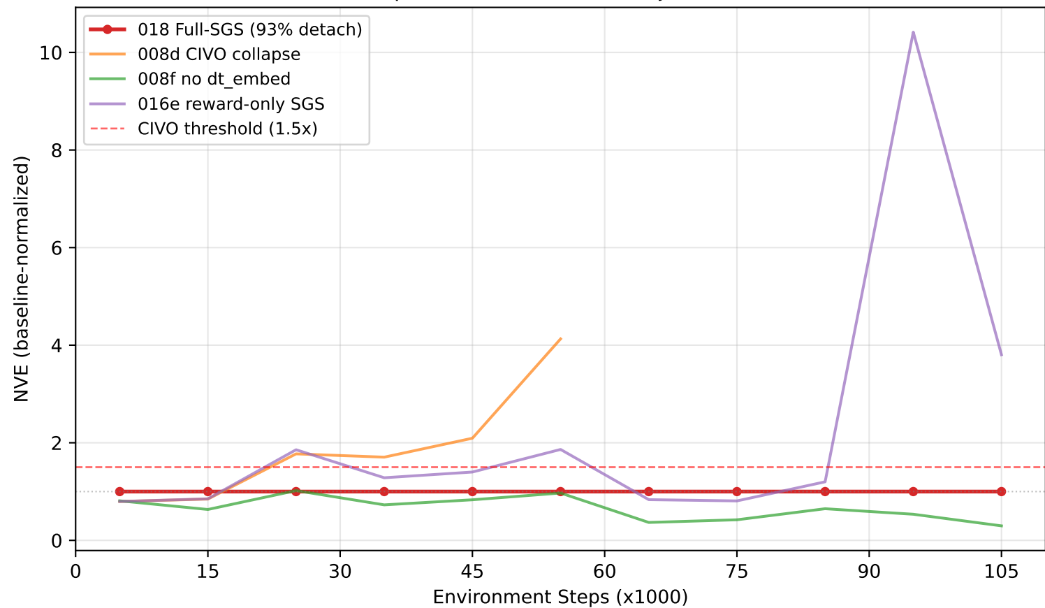
Exp-018 Full-SGS: NVE Trajectories
