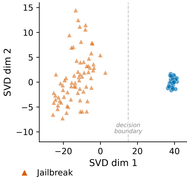
(b) Compressed — clear separation
