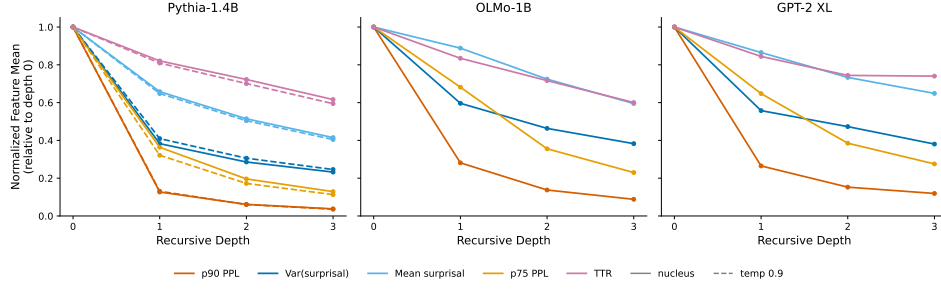
Figure 3: Feature trajectories (normalized to depth 0) across models and strategies. The d=0 \rightarrow d=1 gap dominates; tail features (p90_ppl, p75_ppl) decline most steeply, consistent with tail erosion (§3.5).
