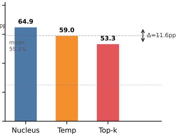
(b) Cross-strategy transfer
