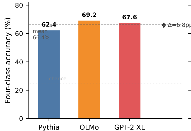
(a) Cross-model transfer
