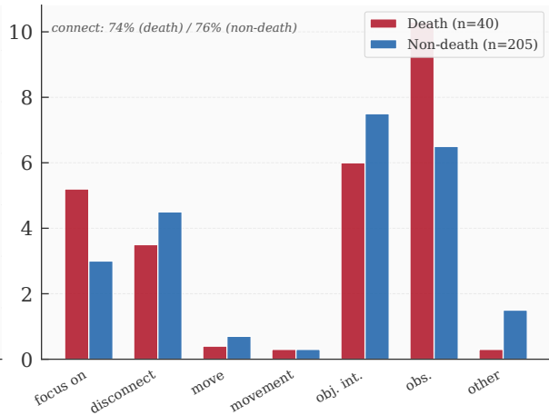
Deterministic
