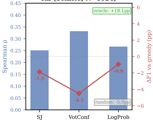
RE (SciERC, N=1024)
