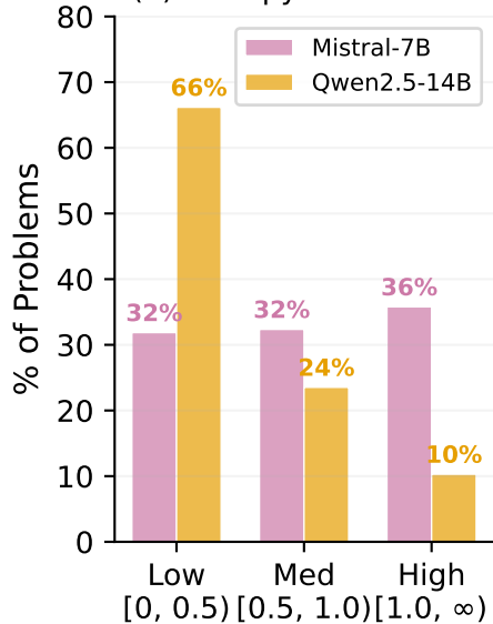
(b) Entropy distribution
