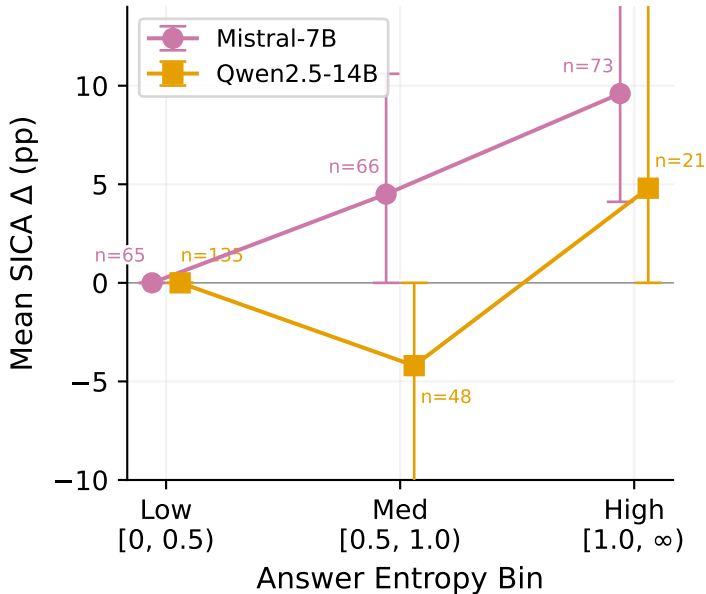
(a) SICA gain by entropy bin
