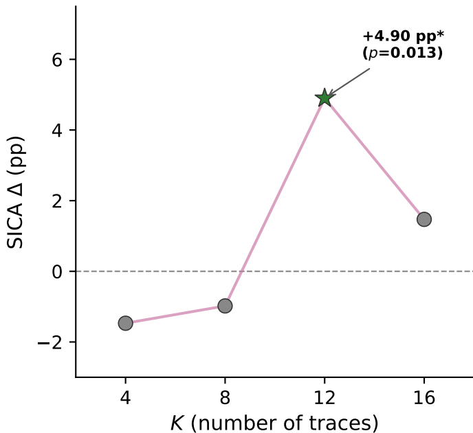
(a) K Sensitivity (Mistral-7B, FOLIO)
