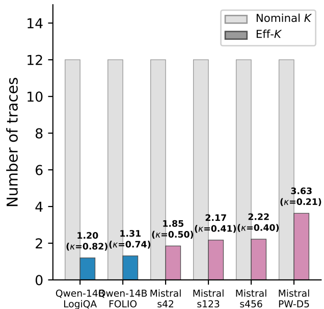
(b) Independence Deficit ( K=12 )
