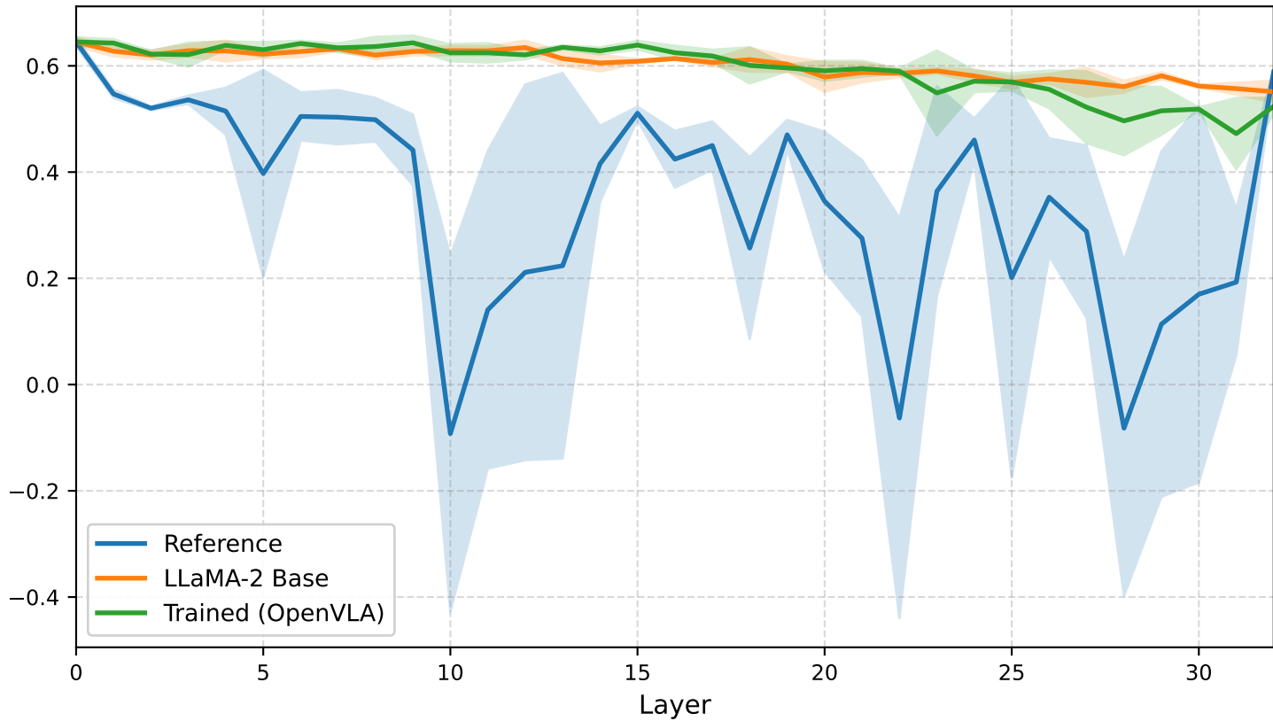
Action R^2 (7-dim)
