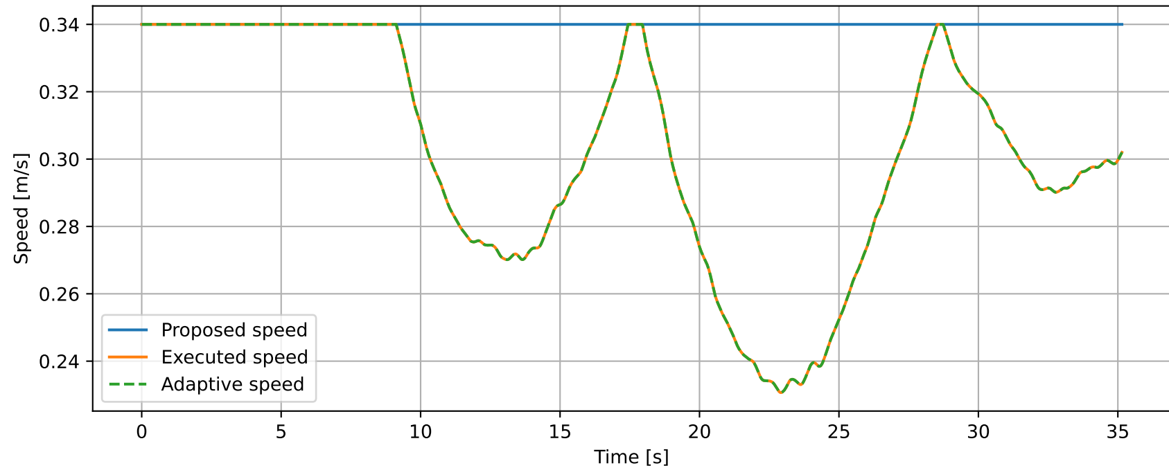
Speed Regulation Under Obstacle-Aware Supervision
