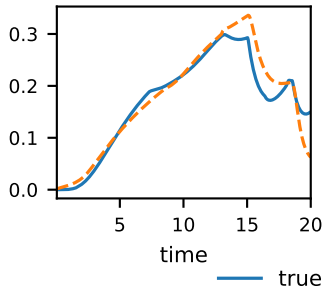
Pyr
