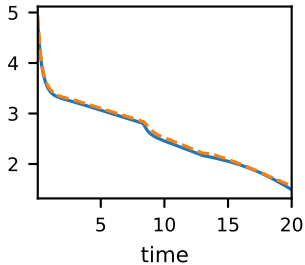
Glc
