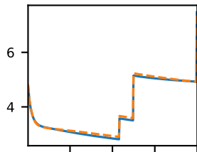
Glc
