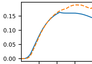
Pyr
