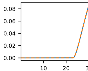
MOF_C
