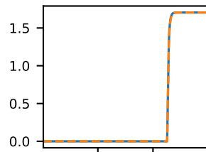
SBU_capped
