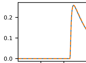
MOF_C
