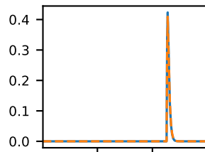
SBU
