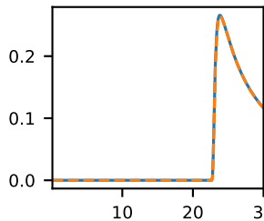
Nuc_A
