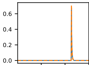
Nuc_A
