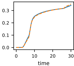
MOF_C
