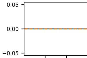
SBU
