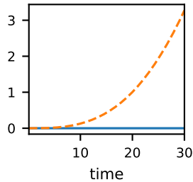
MOF_C
