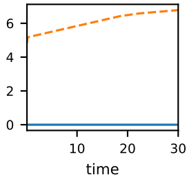
Nuc_A
