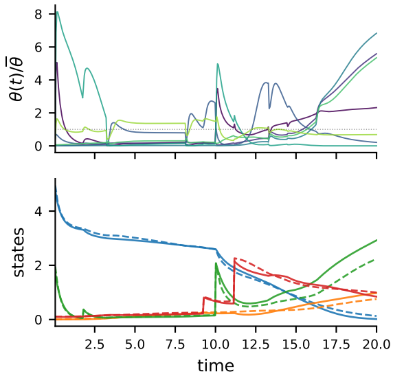
Glycolysis / 4-state
