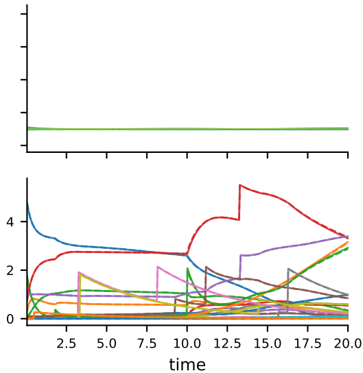
Glycolysis / 22-state
