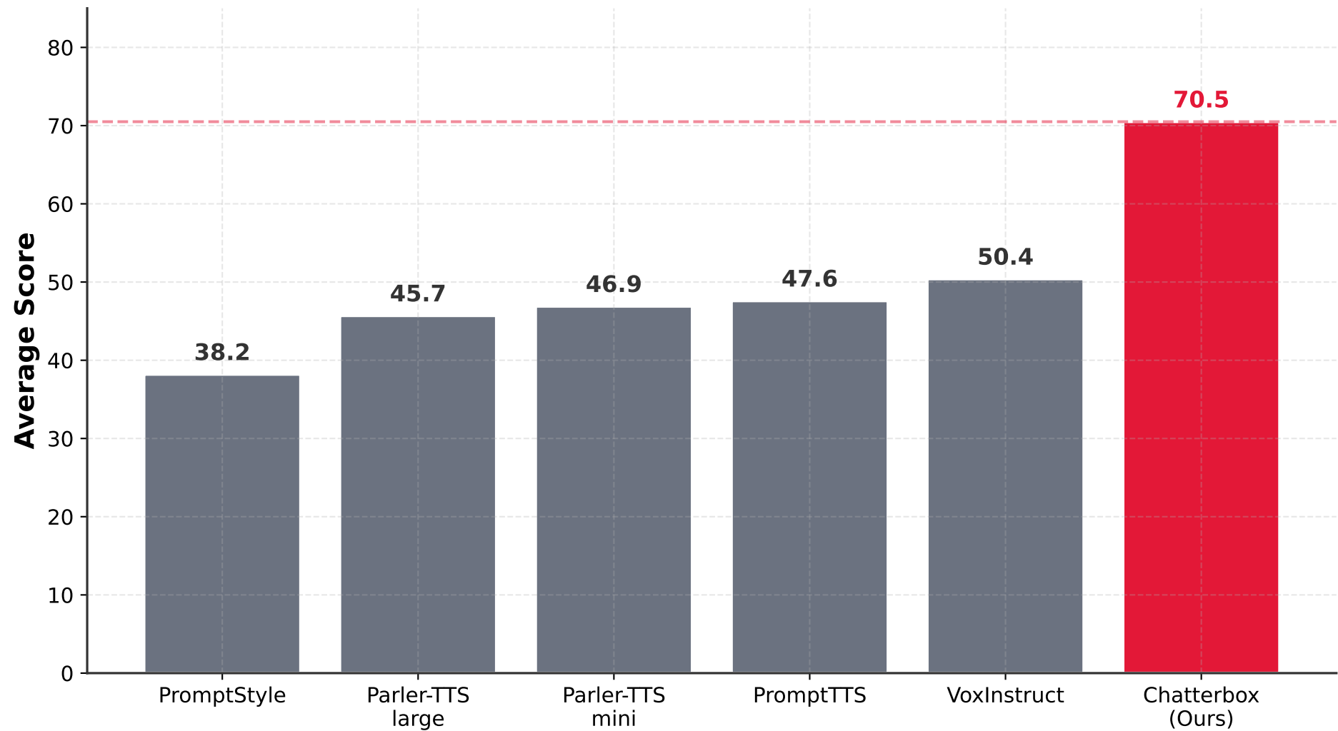
InstructTTSEval - Average Score (Open-Source Models)
