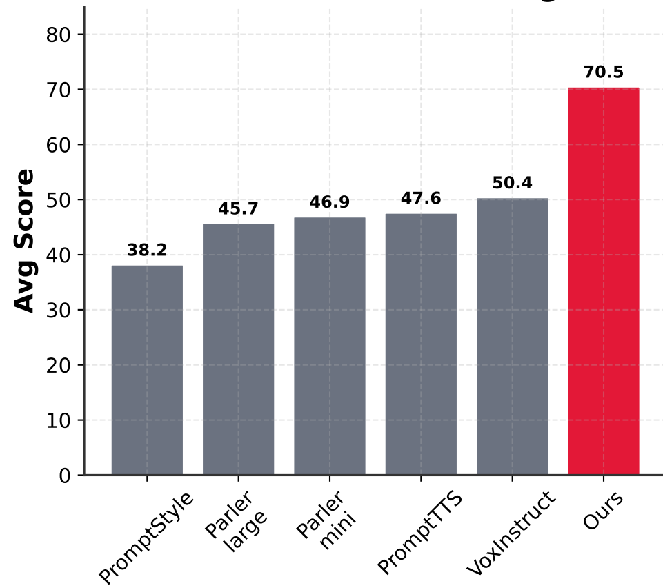
InstructTTEval Average
