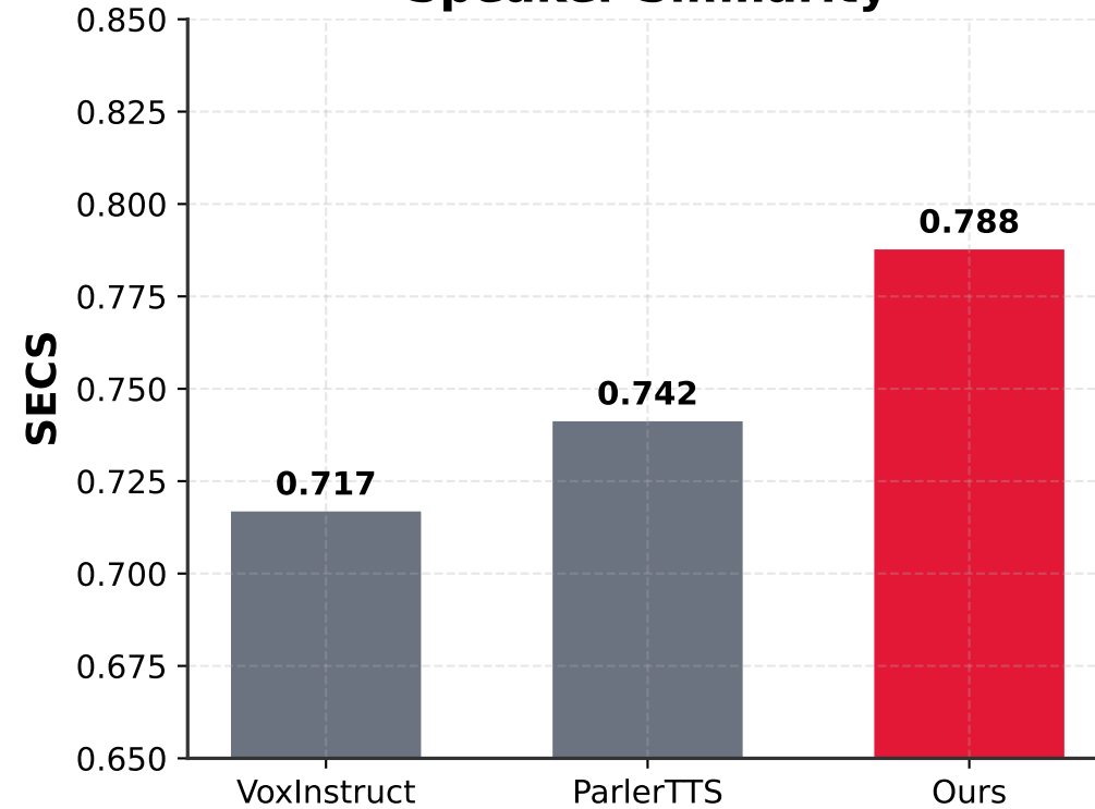
Speaker Similarity
