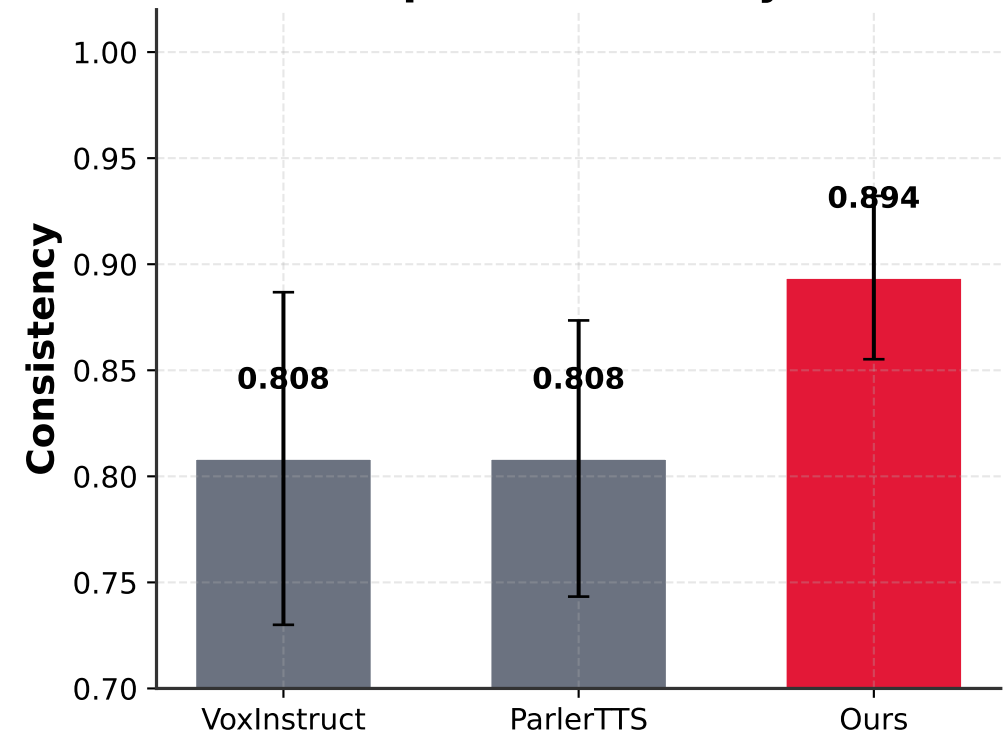
Speaker Stability
