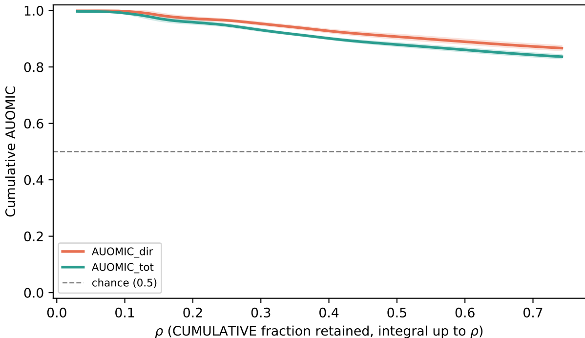
(Beijing, real data) Beijing classification (TIMING): cumulative AUOMIC Cumulative AUOMIC curve (mean \pm 1 std, CV folds)
