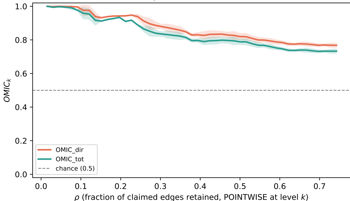
(Beijing, real data) Beijing classification (TIMING): OMIC ranking curve Pointwise ranking curve (mean \pm 1 std, CV folds)
