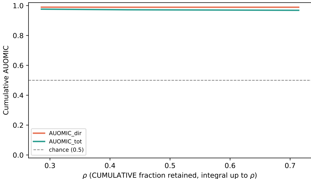
(Beijing, real data) Beijing forecasting (KARMA): cumulative AUOMIC Cumulative AUOMIC curve (mean \pm 1 std, CV folds)
