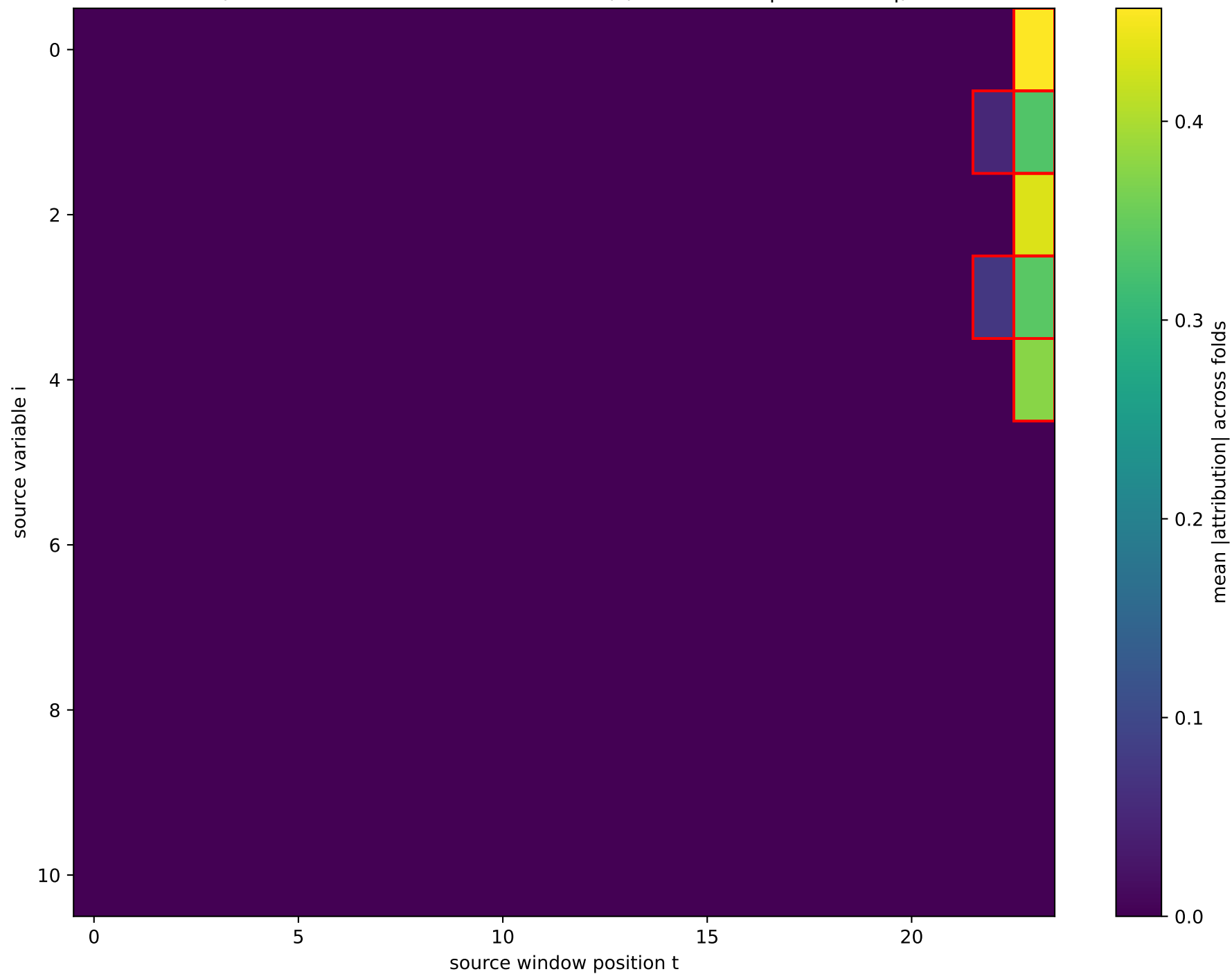
Beijing forecasting (KARMA): claimed edges (red = claimed in \geq 1 of 5 CV fold(s), fold-mean |\text{attribution}| )
