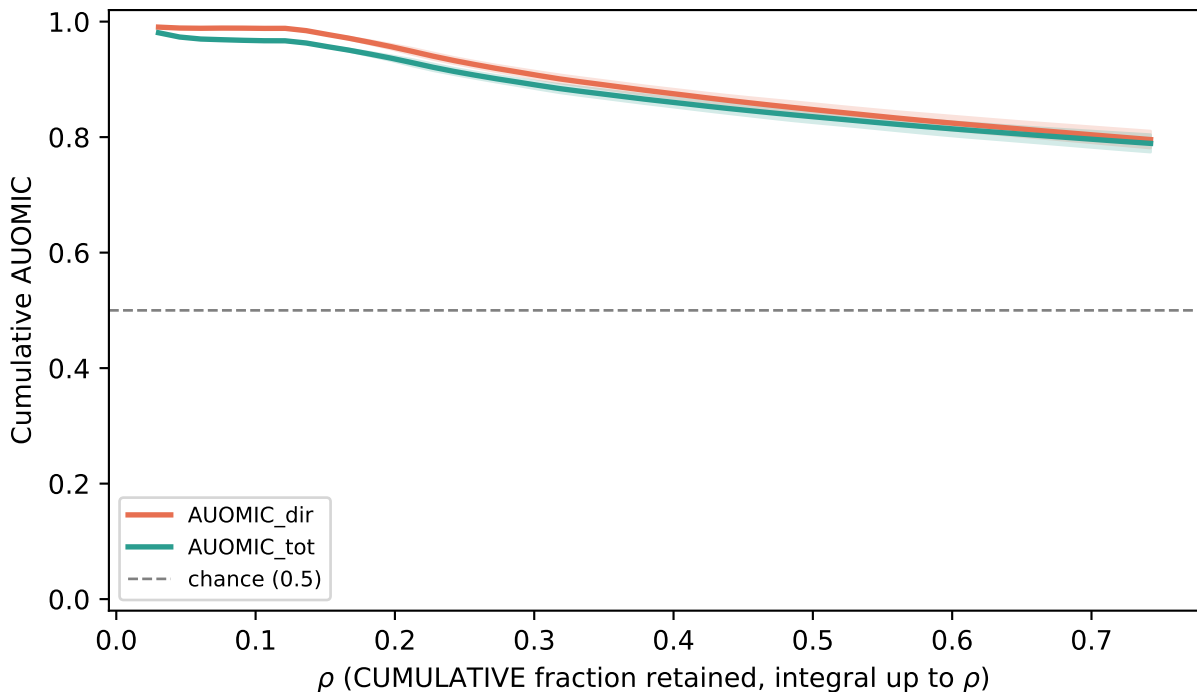
(Beijing, real data) Beijing regression (TimeSHAP): cumulative AUOMIC Cumulative AUOMIC curve (mean \pm 1 std, CV folds)
