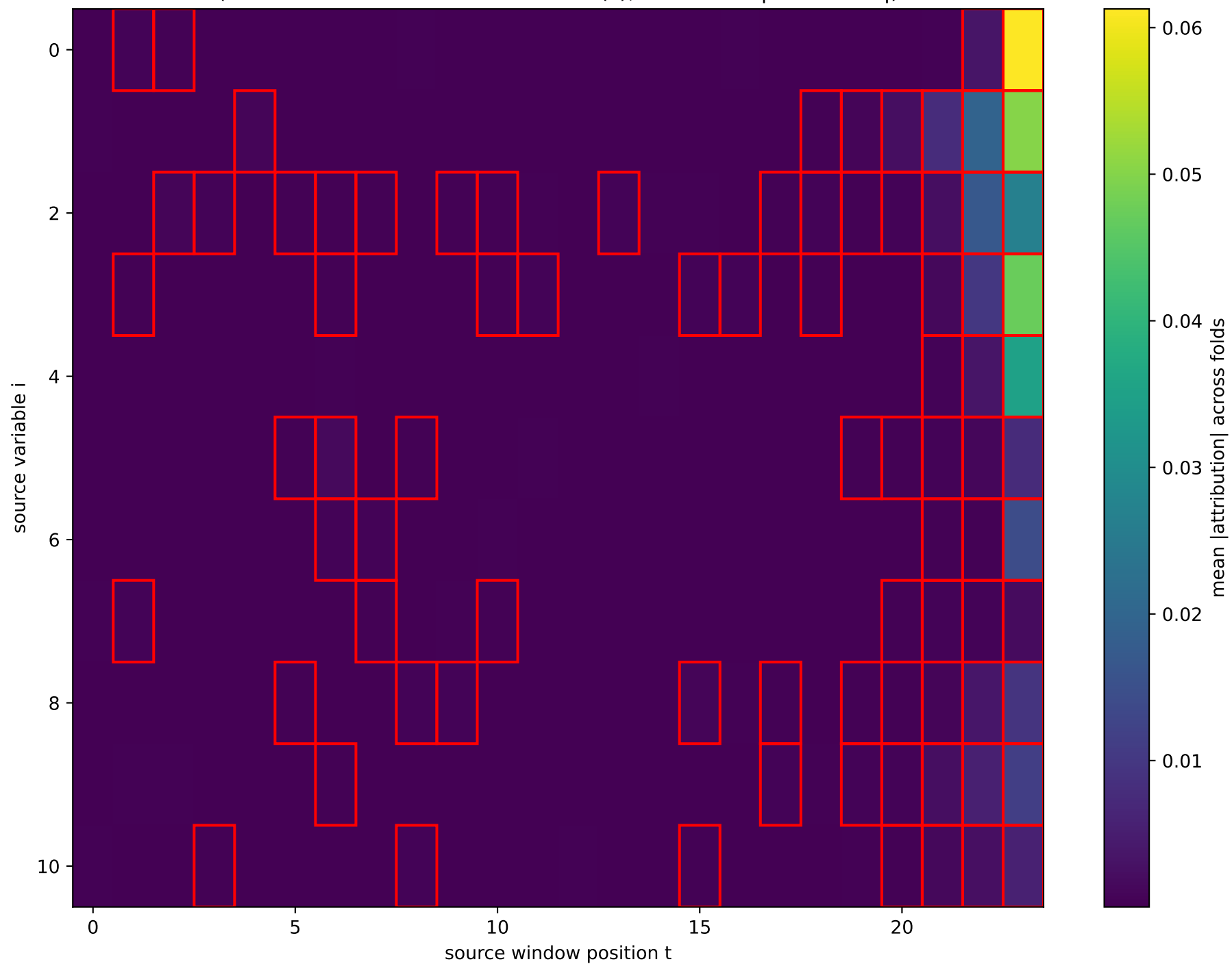
Beijing regression (TimeSHAP): claimed edges (red = claimed in \geq 1 of 5 CV fold(s), fold-mean |\text{attribution}| )
