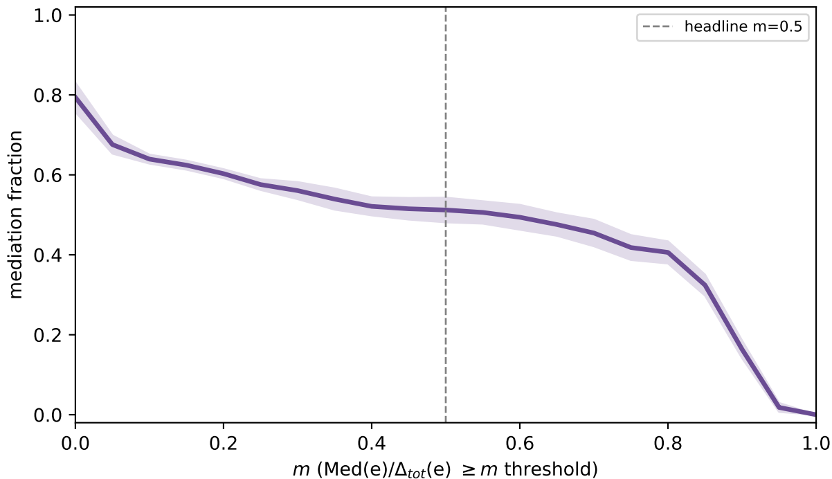
(Beijing, real data) Beijing regression (TimeSHAP): mediation mediation fraction vs. threshold m (mean \pm 1 std, CV folds)
