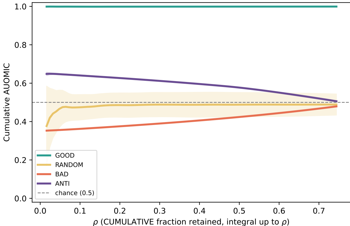
OMIC Metric Validation (synthetic VAR, known ground truth)
