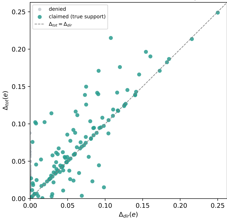
Direct-vs-total effect per candidate edge (synthetic VAR) Med(e) = vertical distance from the diagonal
