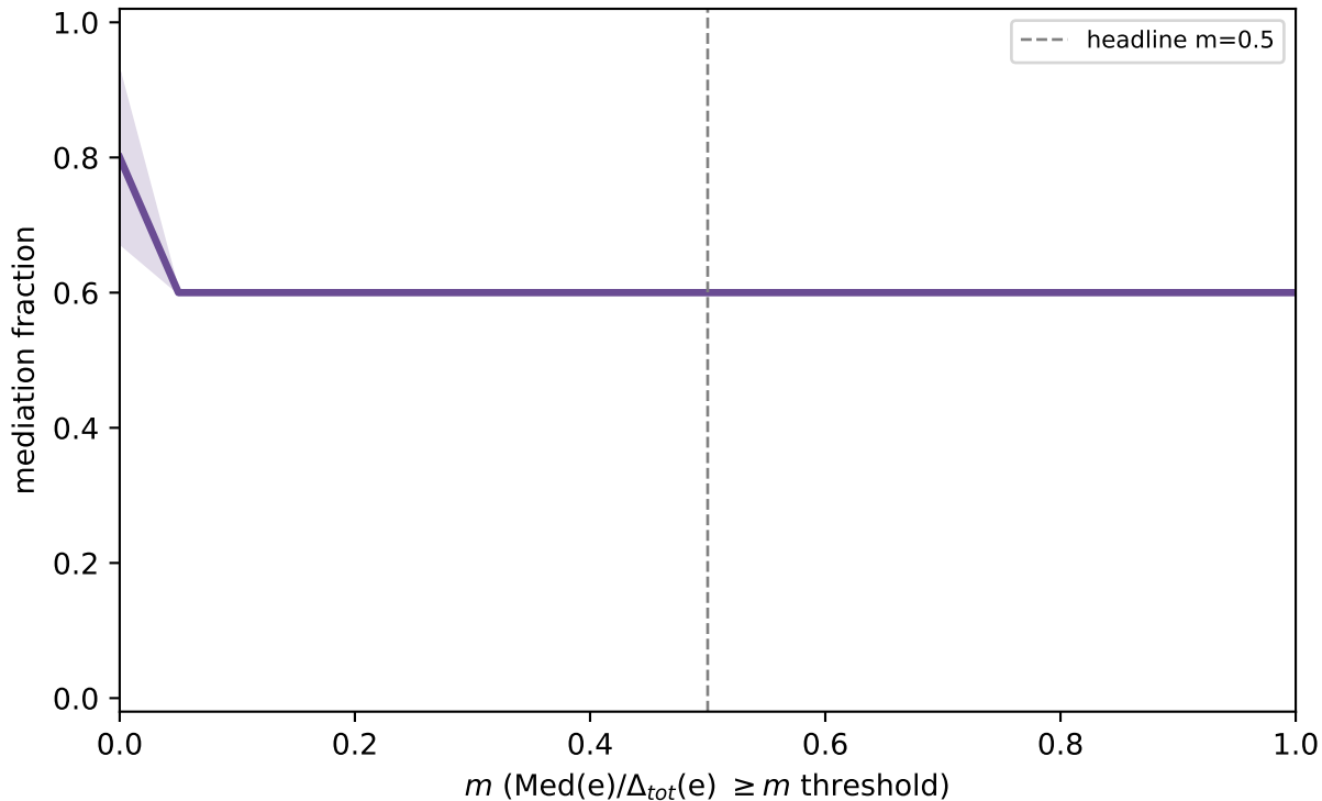
mediation fraction vs. threshold m (the headline number is one point on this curve)
