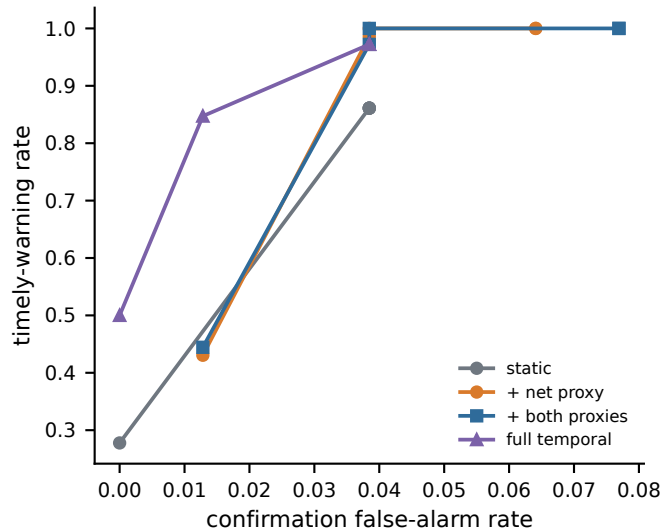
b Fixed scores, calibration-budget sensitivity
