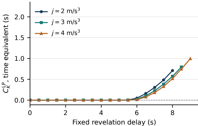
(a) Initial speed 22.2 m/s
