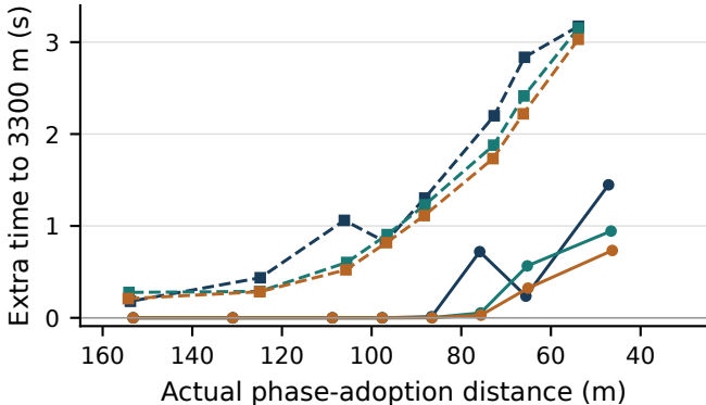
(a) Initial speed 22.2 m/s
