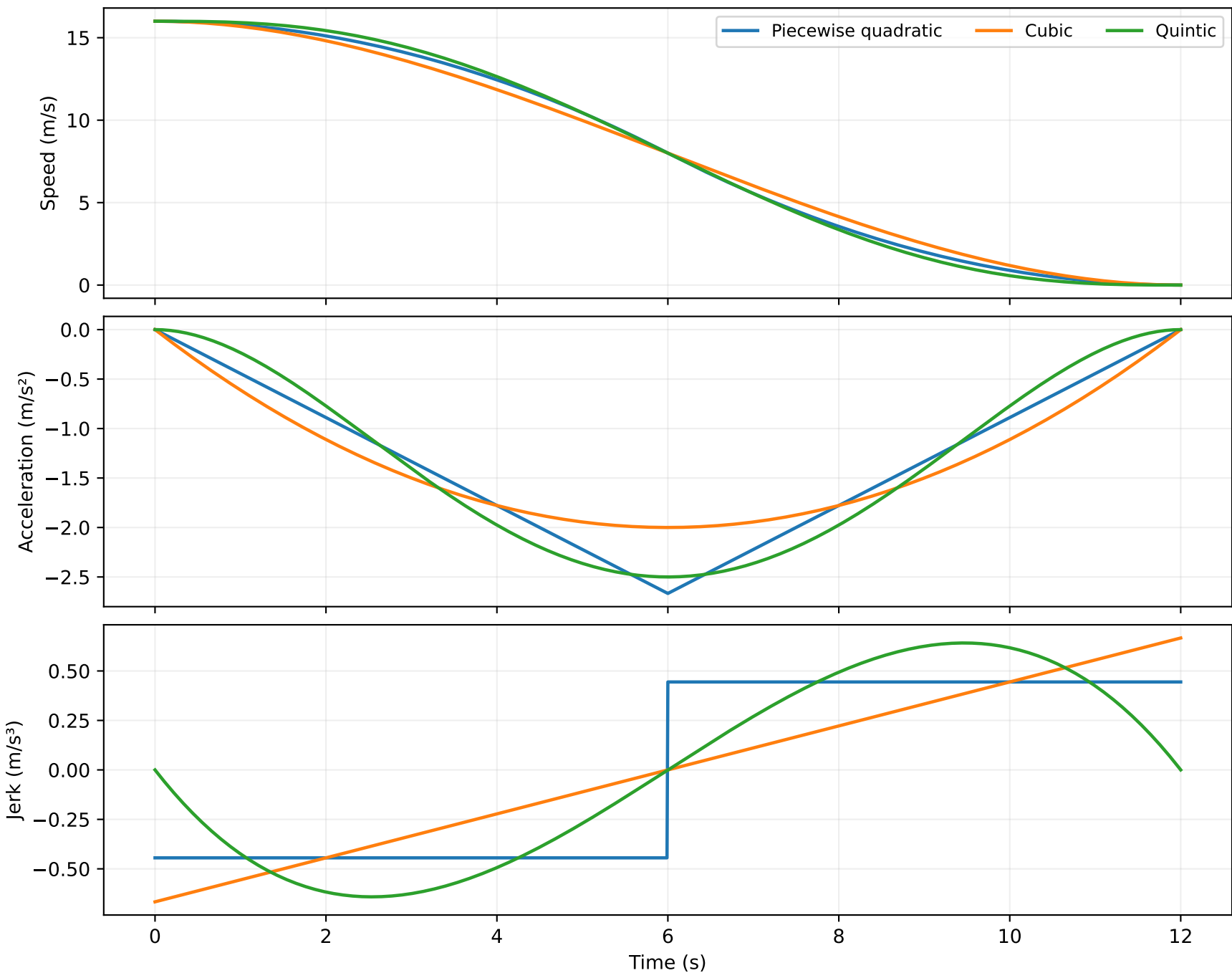
Same stop: 16 \rightarrow 0 m/s, 12 s, 96 m, zero endpoint acceleration Curve shape trades peak jerk against integrated squared jerk
