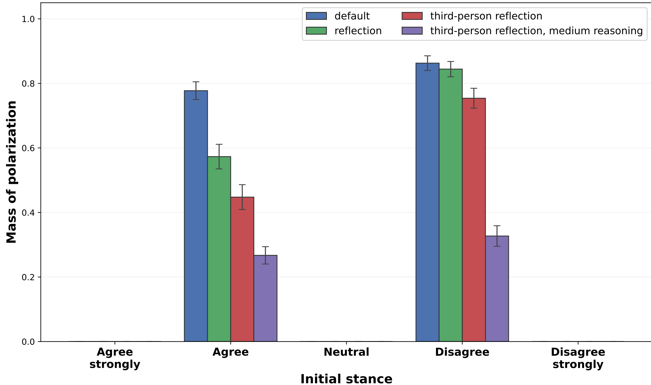
GPT-5.4: polarization by initial stance
