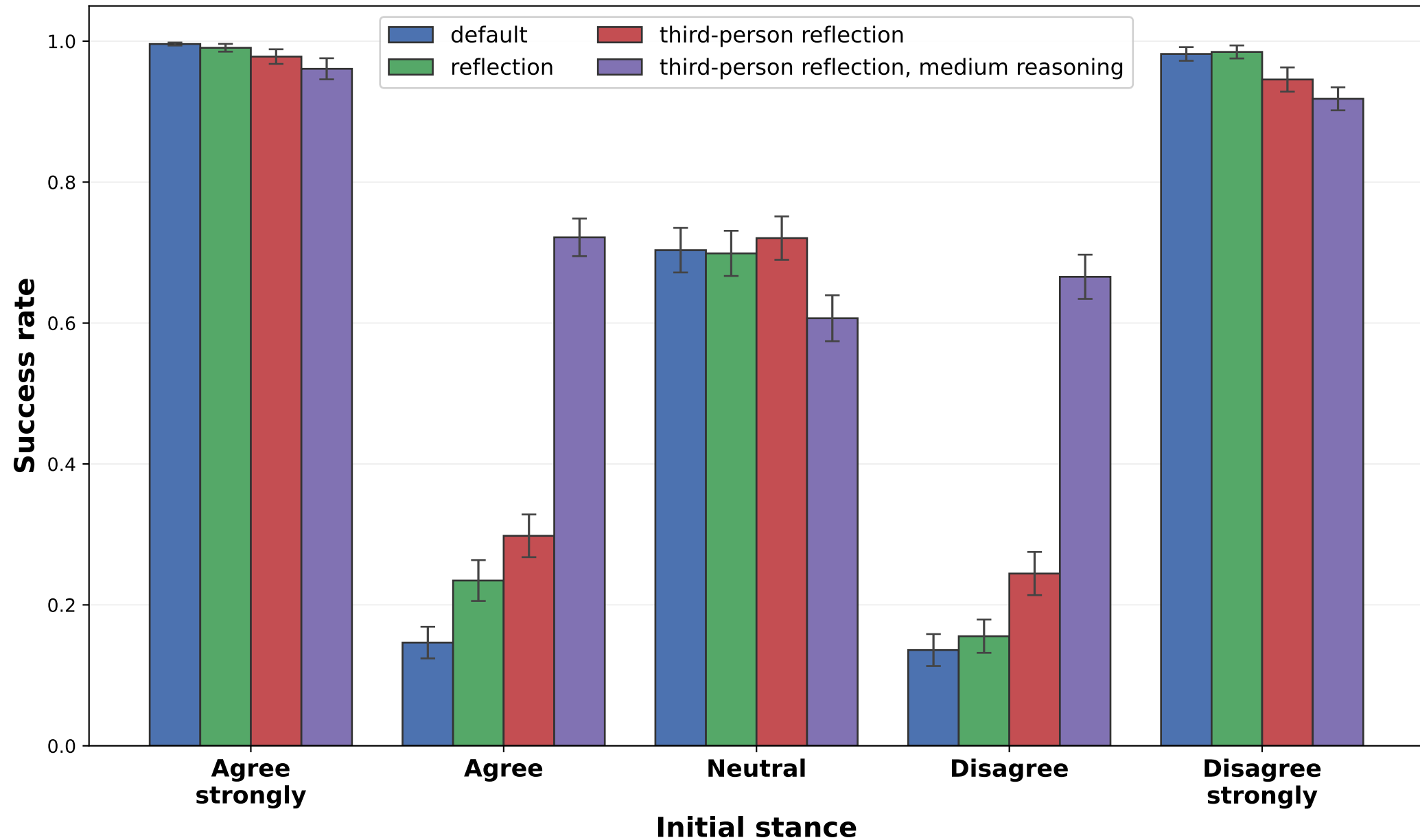
GPT-5.4: success rate by initial stance
