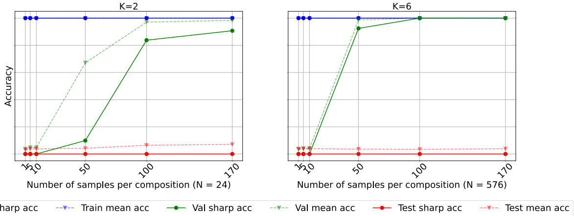
Figure 28. Effect of number of samples per composition (uniform benchmark, direct model): We observe that for a low number of training samples, the train/val gap is high and the model struggles to generalize to training compositions with novel inputs. The train-val gap reduces as the number of samples increases. Test accuracies remain 0%, as expected.
