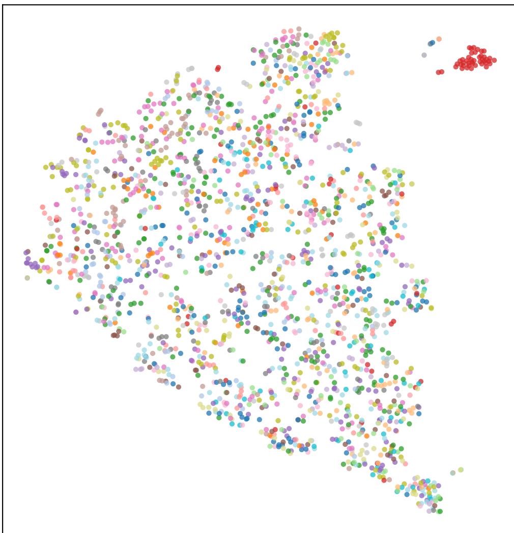
Barlow Twins
