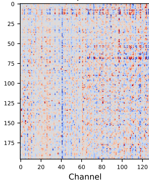
MHLA_L Rank=128 | EffRank=84.9
